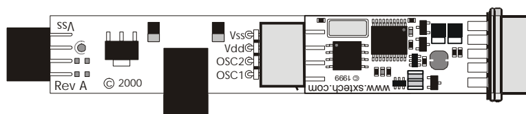
Figure 2: KeyRing Connection Diagram
